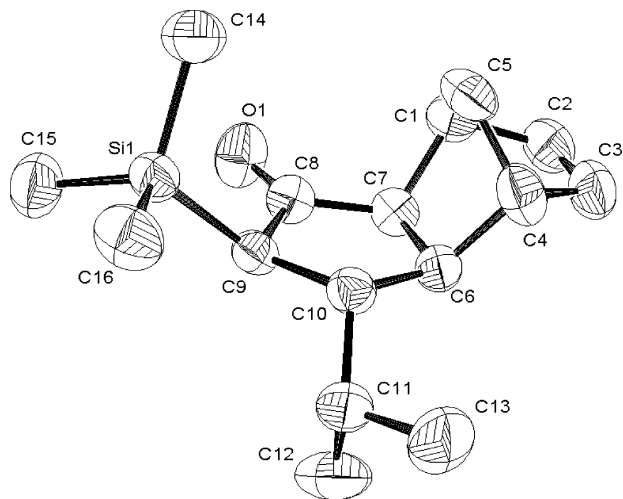
FIGURE 5. Ortep drawing of 22c showing 50% probability ellipsoids.
